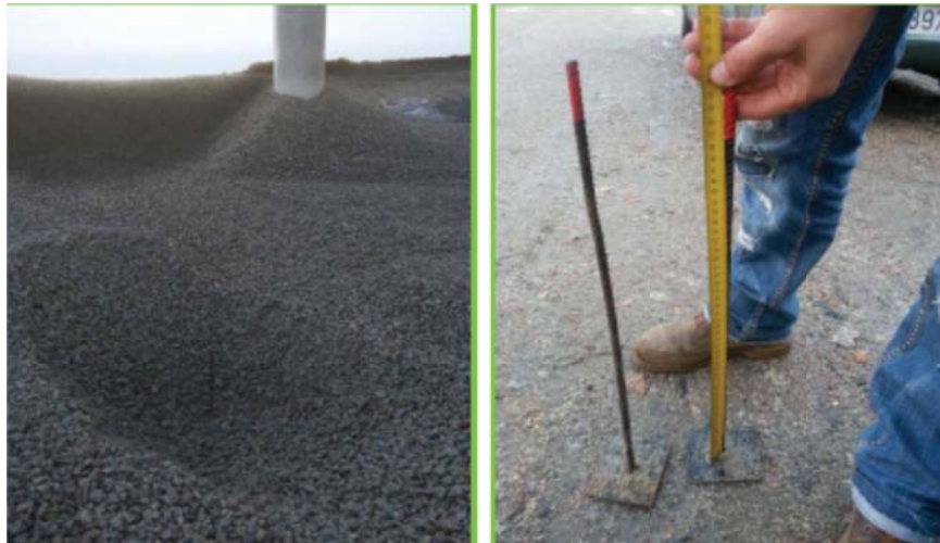
Figure 42: Thickness of gravel layer
